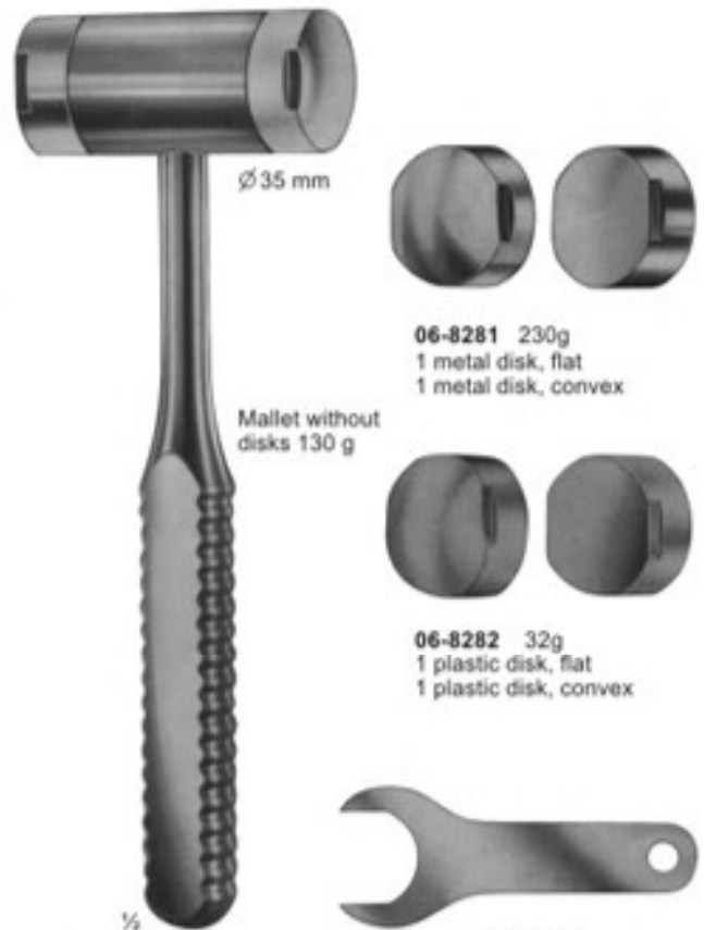
06-8280 - 06-8283 WAGNER complete with: 1 pair of metal disks ( 06-8281 ) and 1 pair of plastic disks ( 06-8282 ) and 1 wrench ( 06-8283 ) 235 mm
