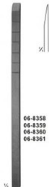
COTTLE 06-8358 - 06-8361 Chisel-Osteotomes with depth markings 180 mm
